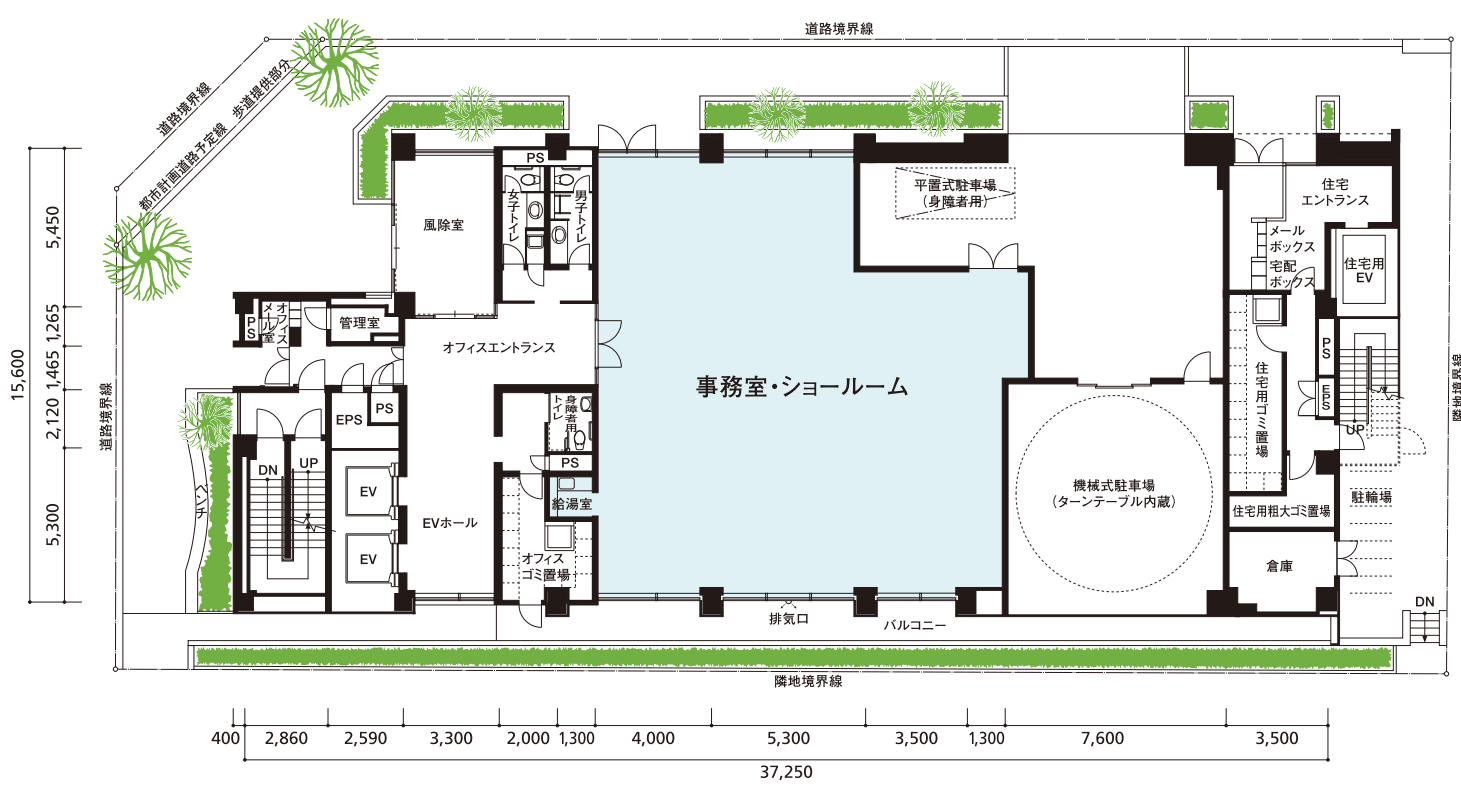
1階平面図 1st Floor
